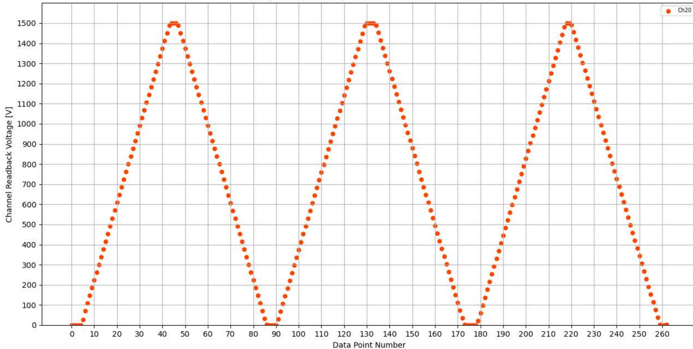
Voltage Ramp Test (Python) Bd #173, Slot #9, Ch #20
