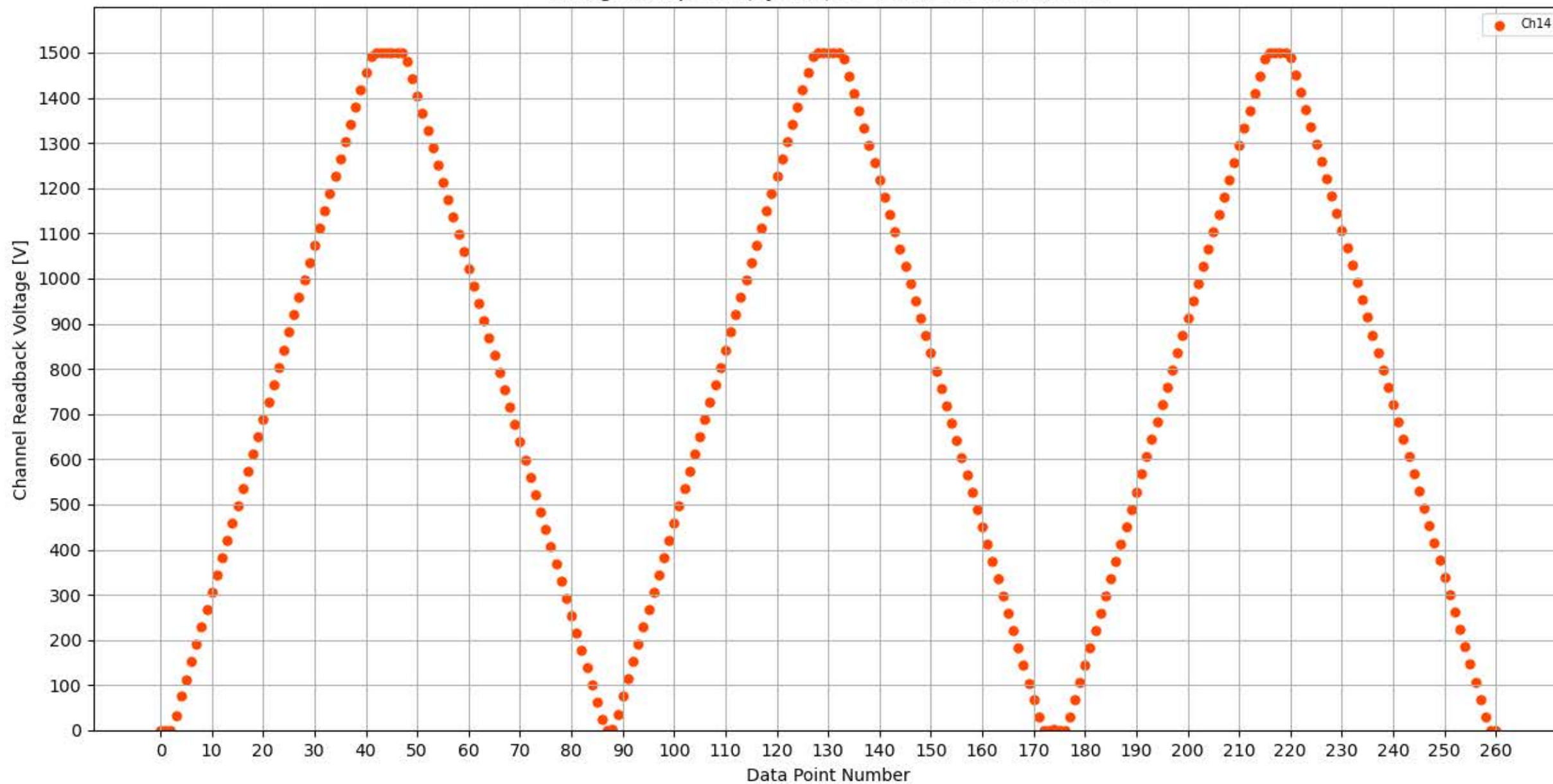
Voltage Ramp Test (Python) Bd #173, Slot #9, Ch #14
