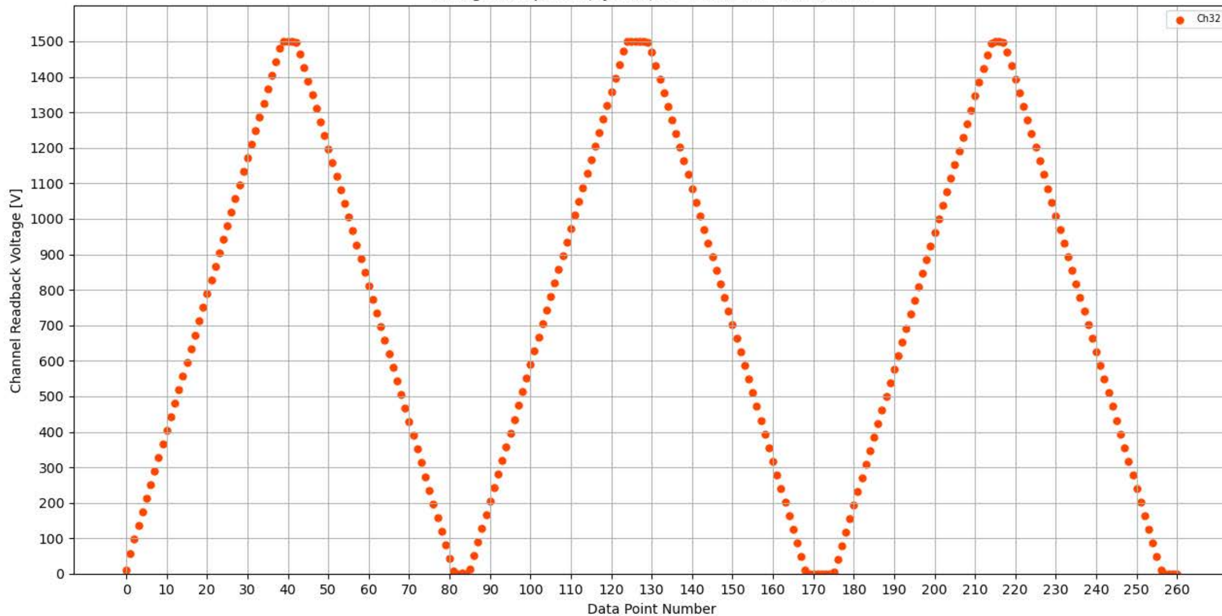
Voltage Ramp Test (Python) Bd #173, Slot #9, Ch #32
