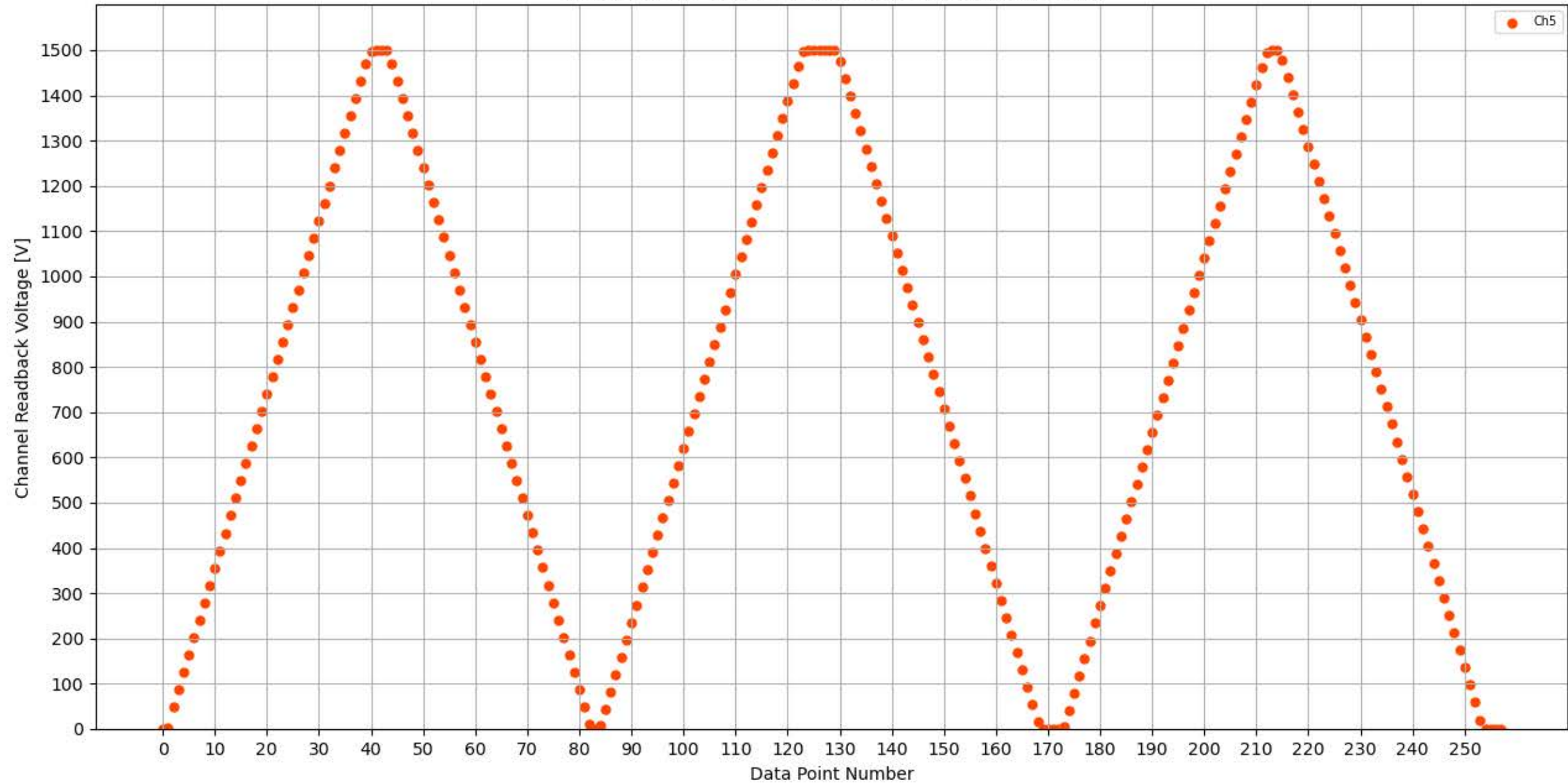
Voltage Ramp Test (Python) Bd #173, Slot #9, Ch #5
