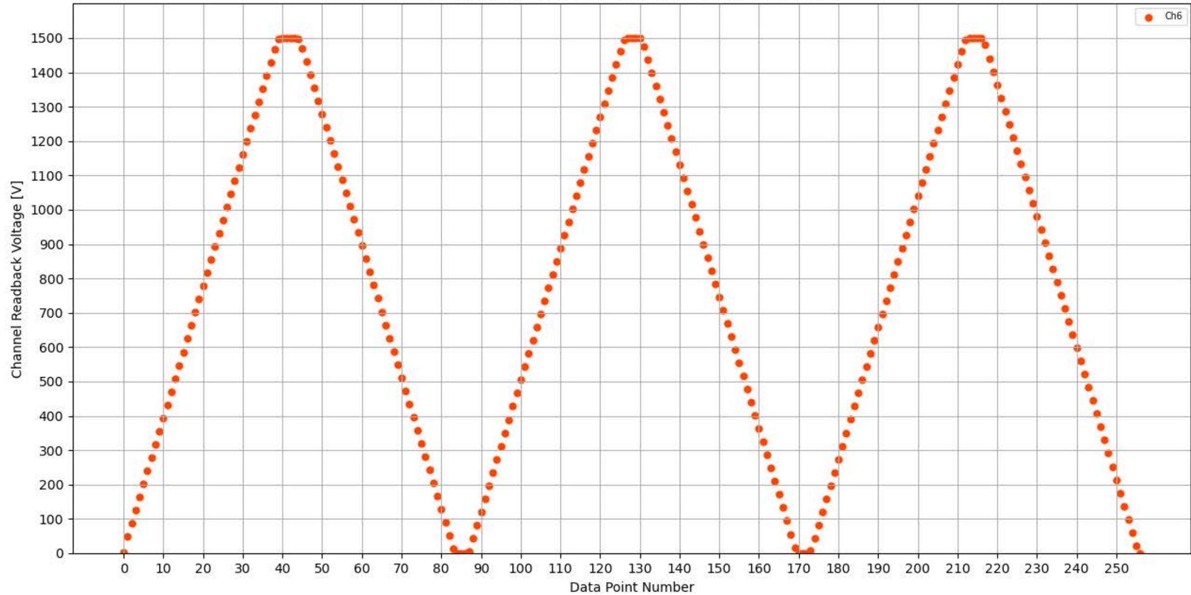
Voltage Ramp Test (Python) Bd #173, Slot #9, Ch #6
