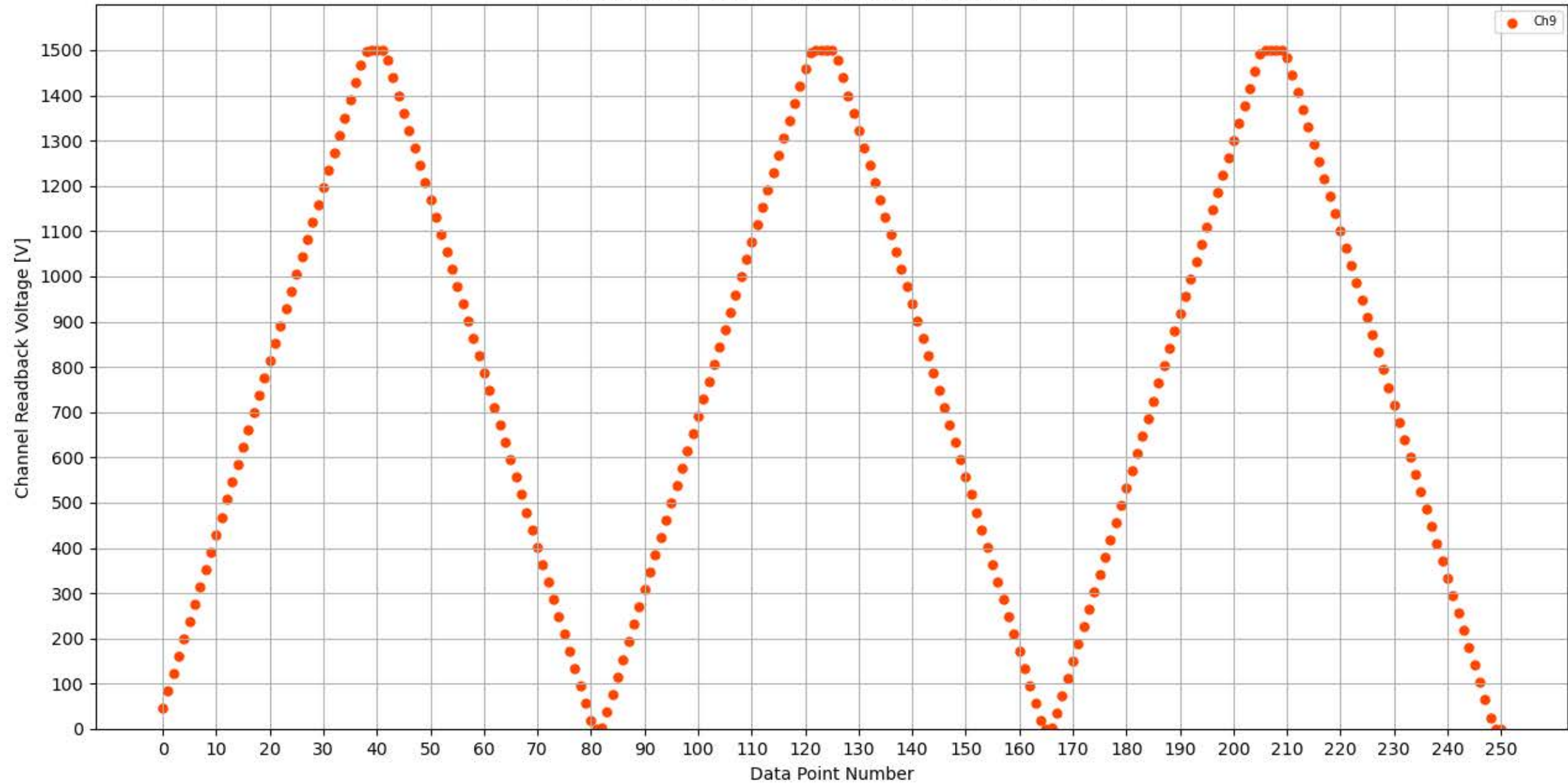
Voltage Ramp Test (Python) Bd #173, Slot #9, Ch #9
