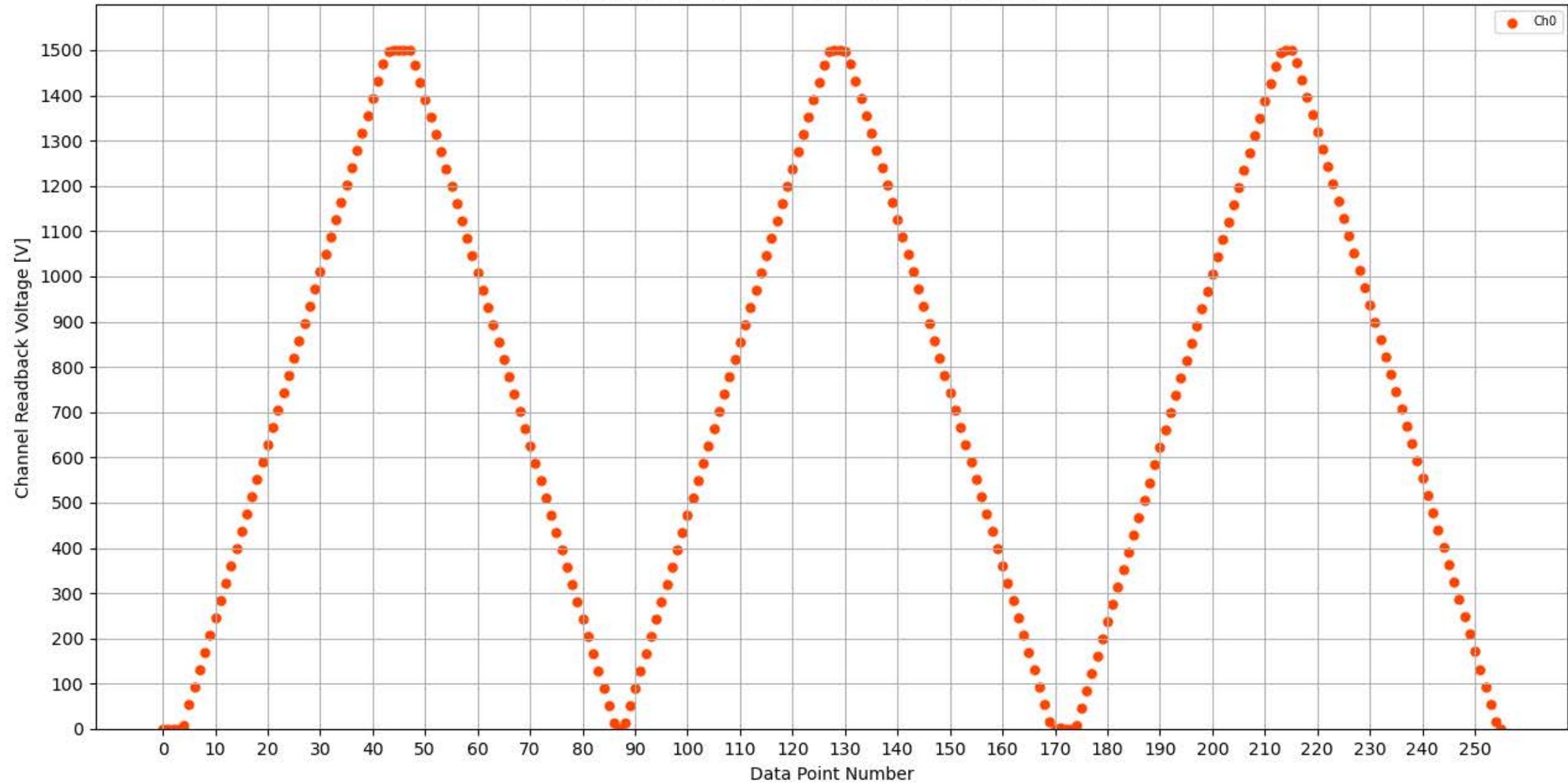
Voltage Ramp Test (Python) Bd #173, Slot #9, Ch #0
