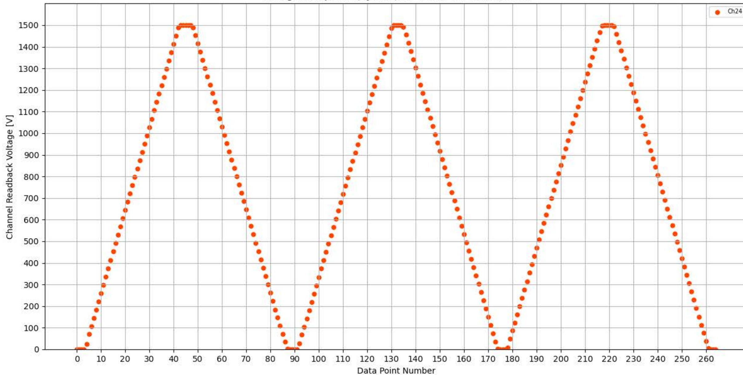
Voltage Ramp Test (Python) Bd #173, Slot #9, Ch #24
