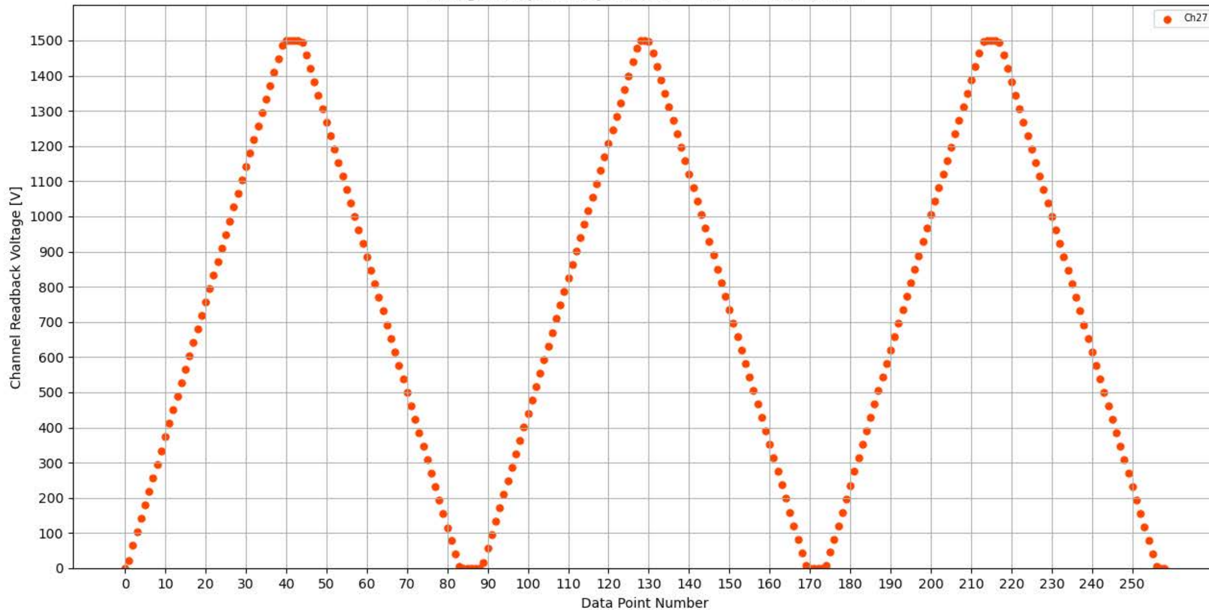
Voltage Ramp Test (Python) Bd #173, Slot #9, Ch #27
