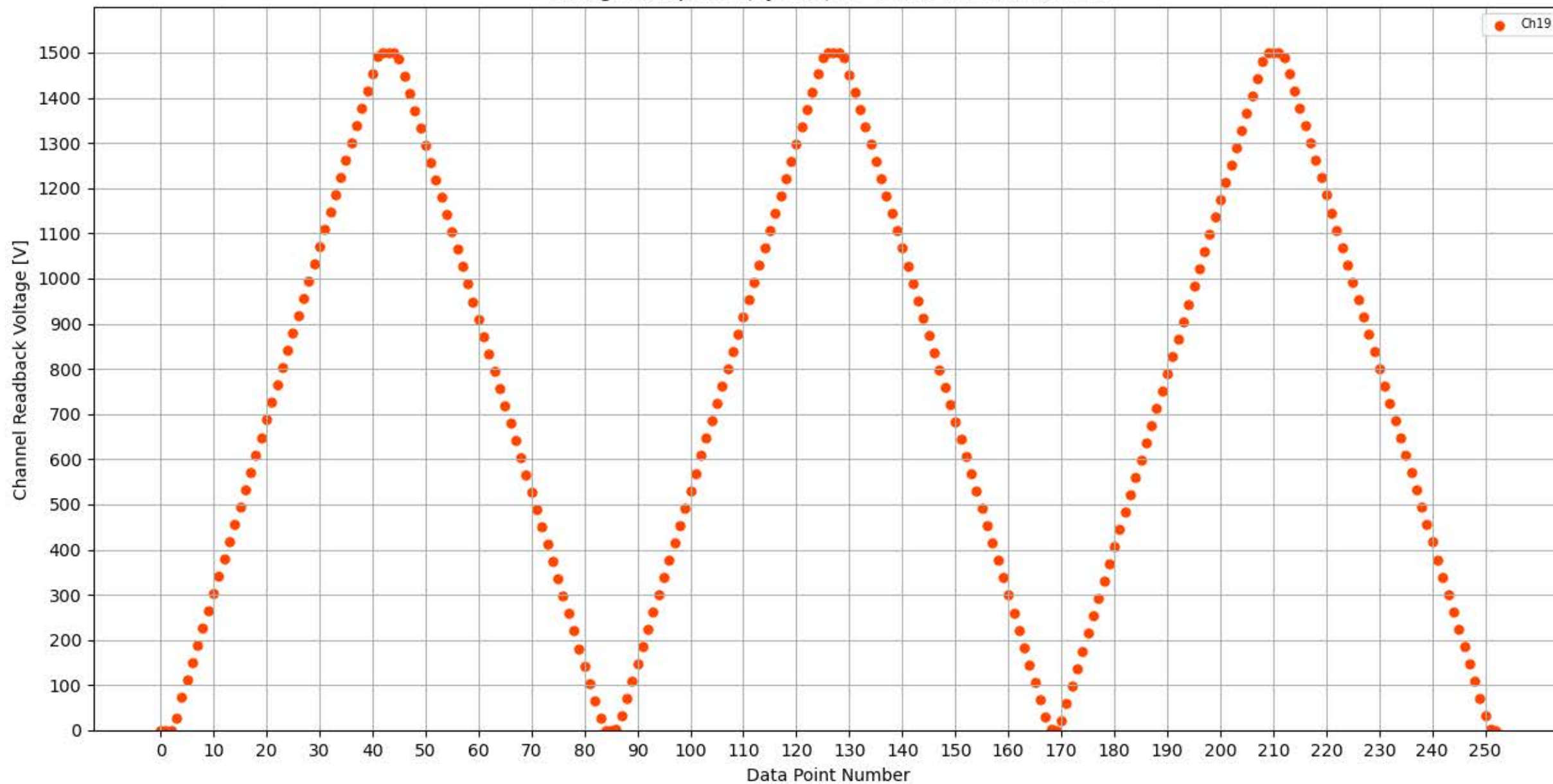
Voltage Ramp Test (Python) Bd #173, Slot #9, Ch #19
