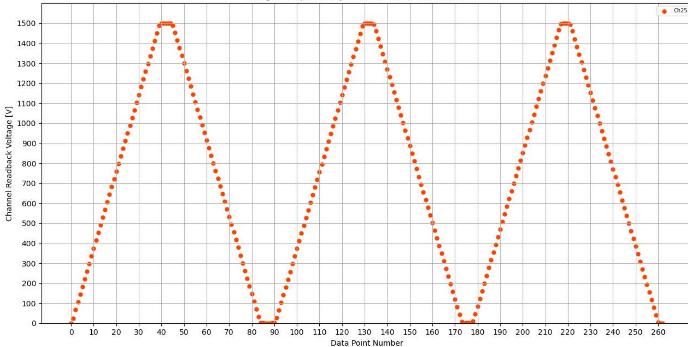
Voltage Ramp Test (Python) Bd #173, Slot #9, Ch #25
