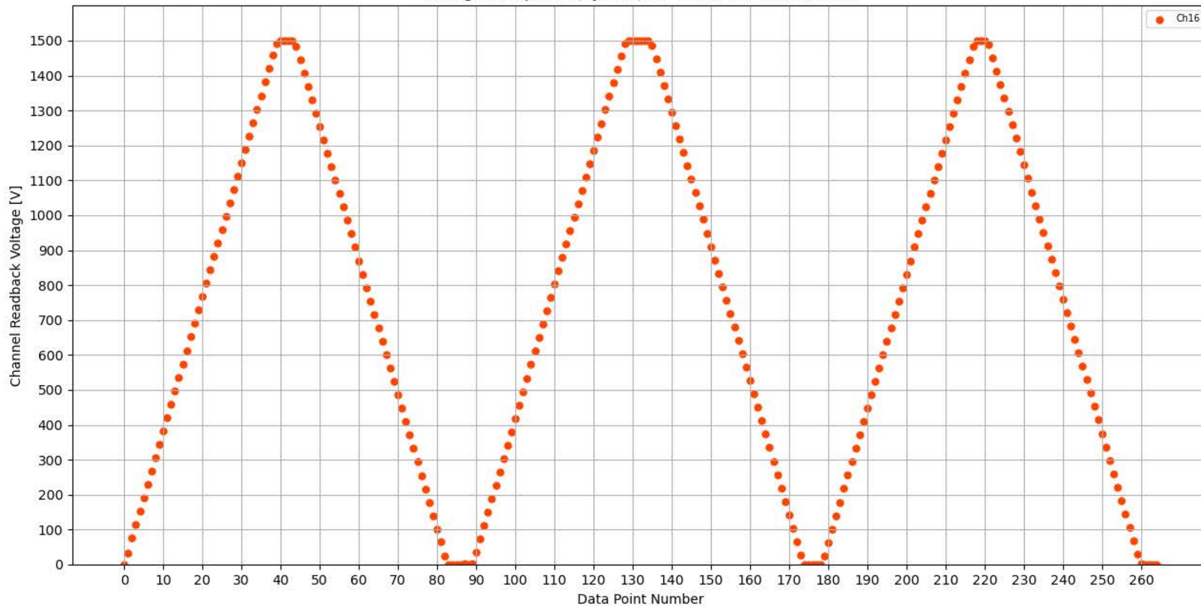
Voltage Ramp Test (Python) Bd #173, Slot #9, Ch #16
