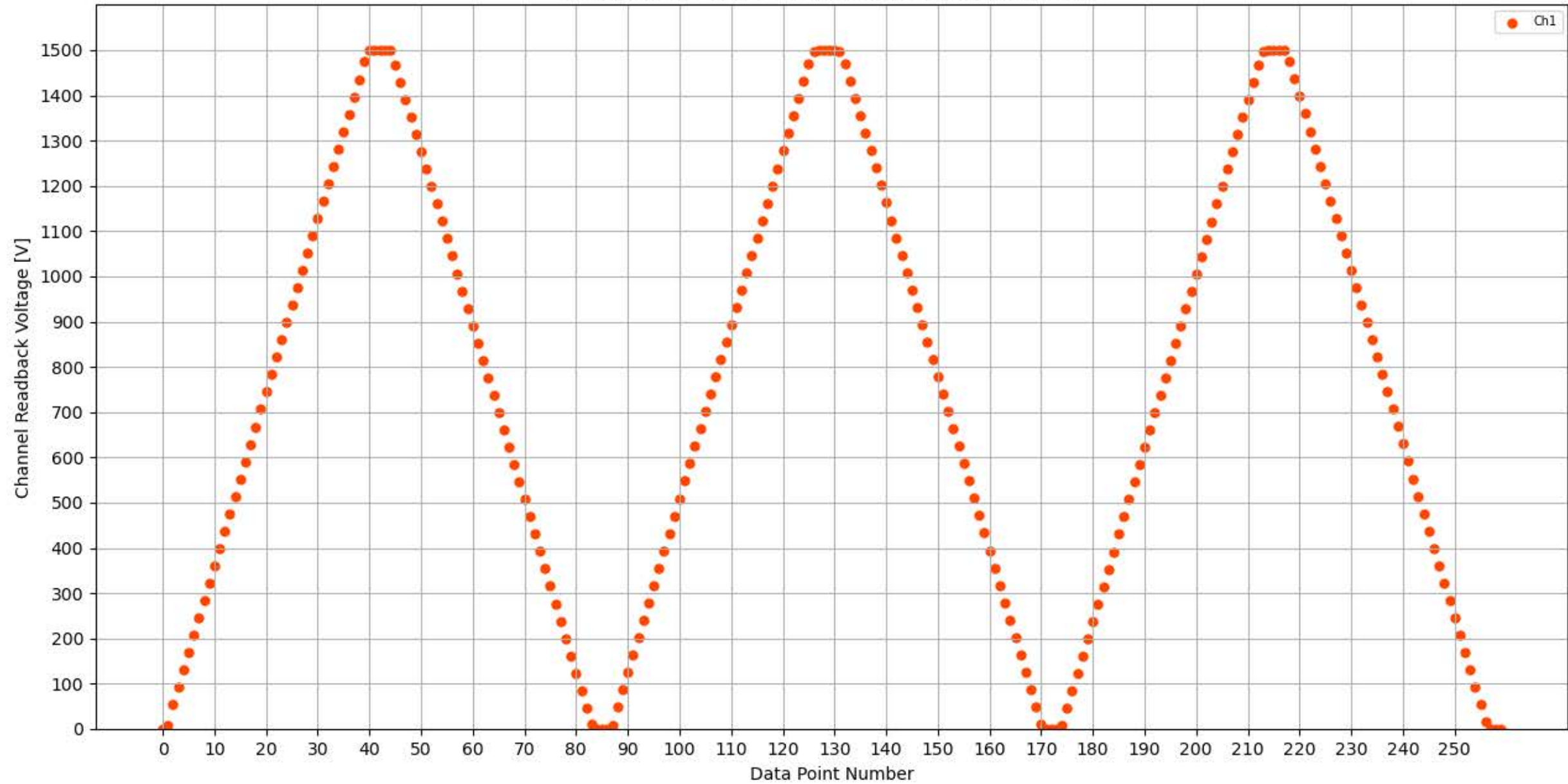
Voltage Ramp Test (Python) Bd #173, Slot #9, Ch #1
