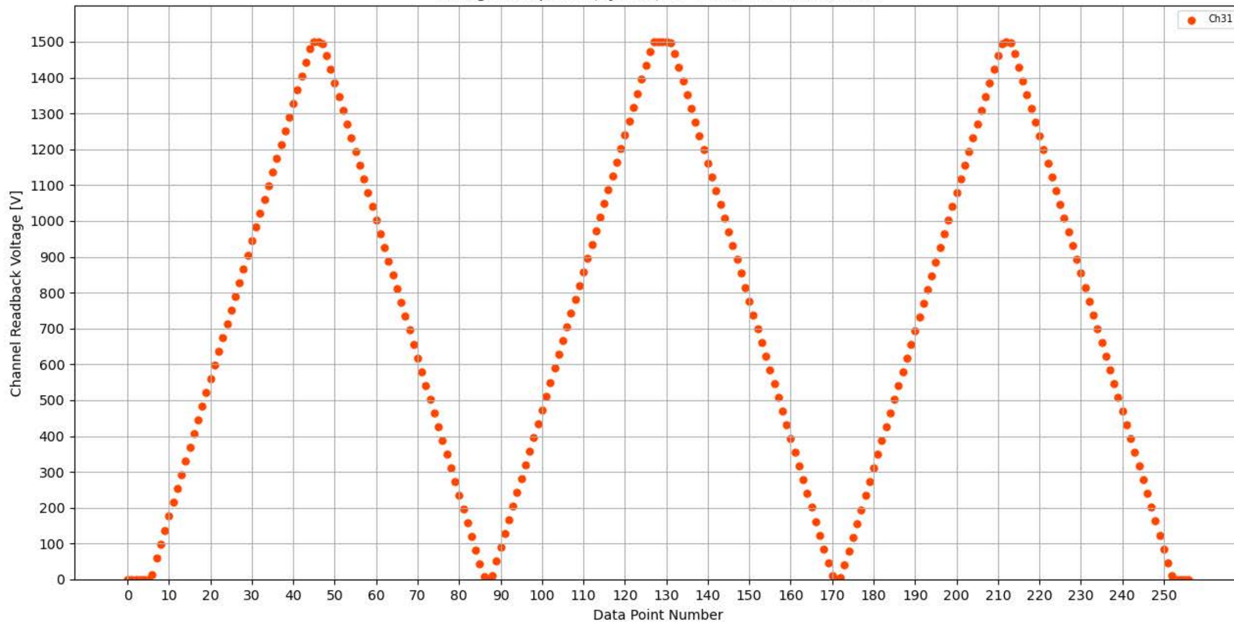
Voltage Ramp Test (Python) Bd #173, Slot #9, Ch #31
