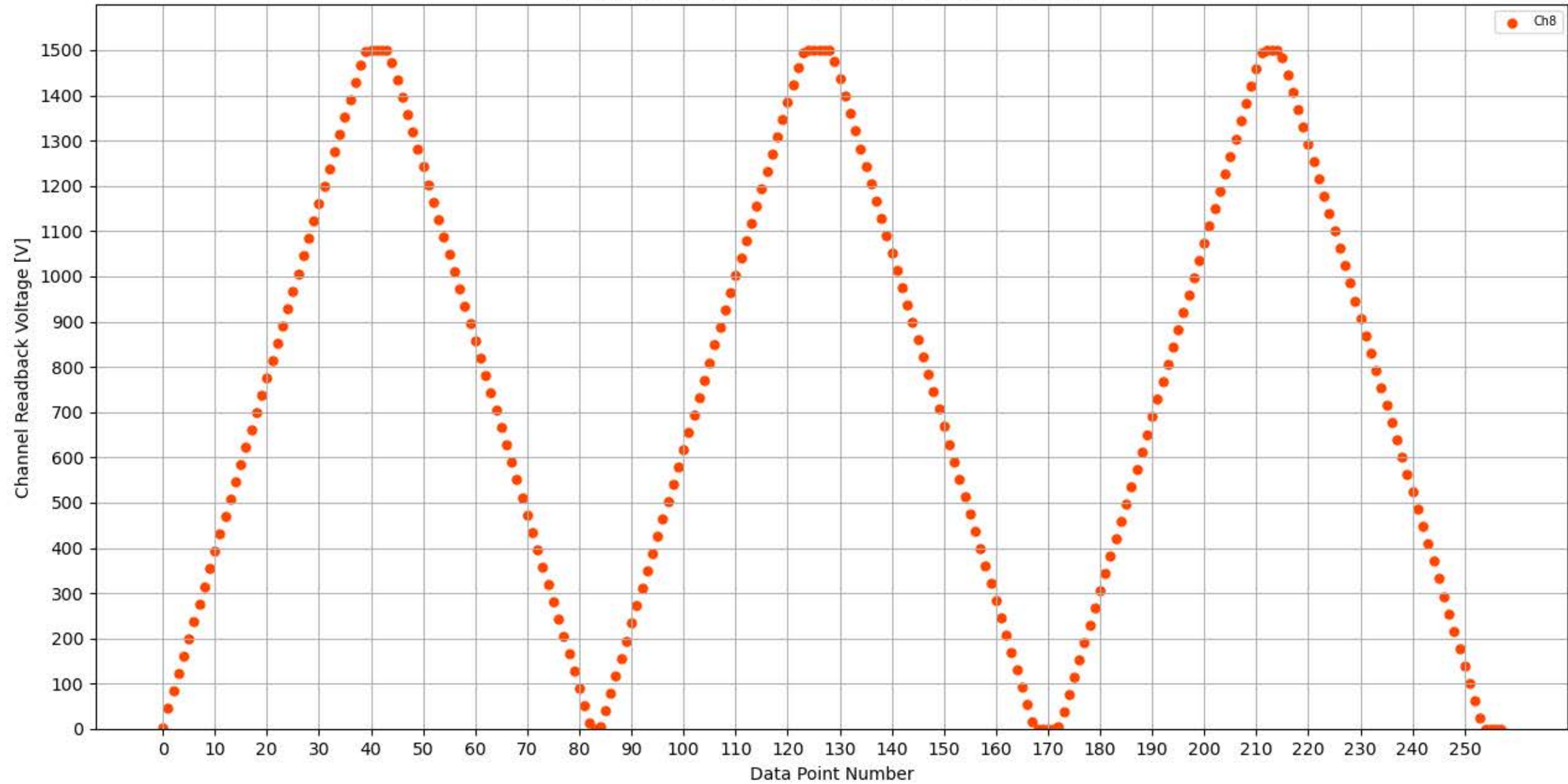
Voltage Ramp Test (Python) Bd #173, Slot #9, Ch #8
