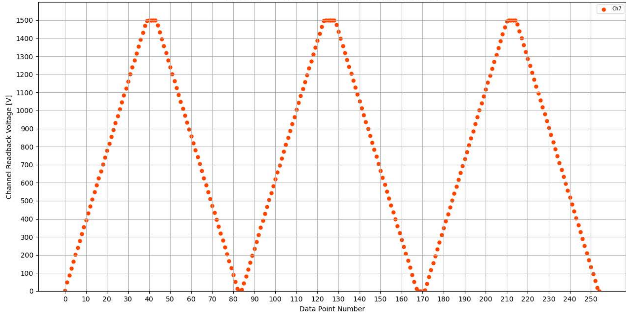
Voltage Ramp Test (Python) Bd #173, Slot #9, Ch #7
