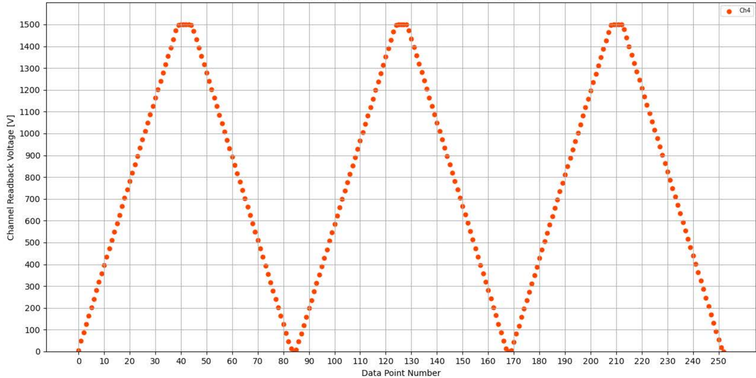
Voltage Ramp Test (Python) Bd #173, Slot #9, Ch #4
