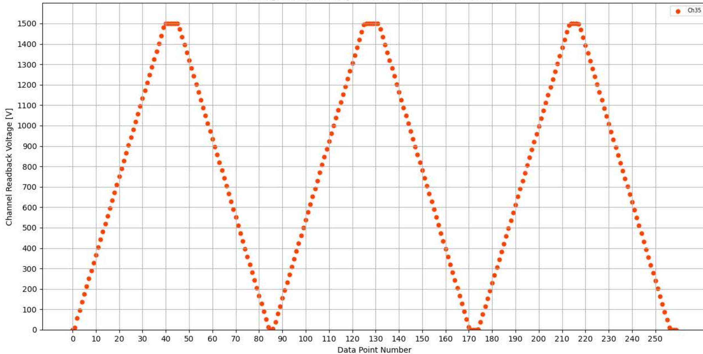
Voltage Ramp Test (Python) Bd #173, Slot #9, Ch #35
