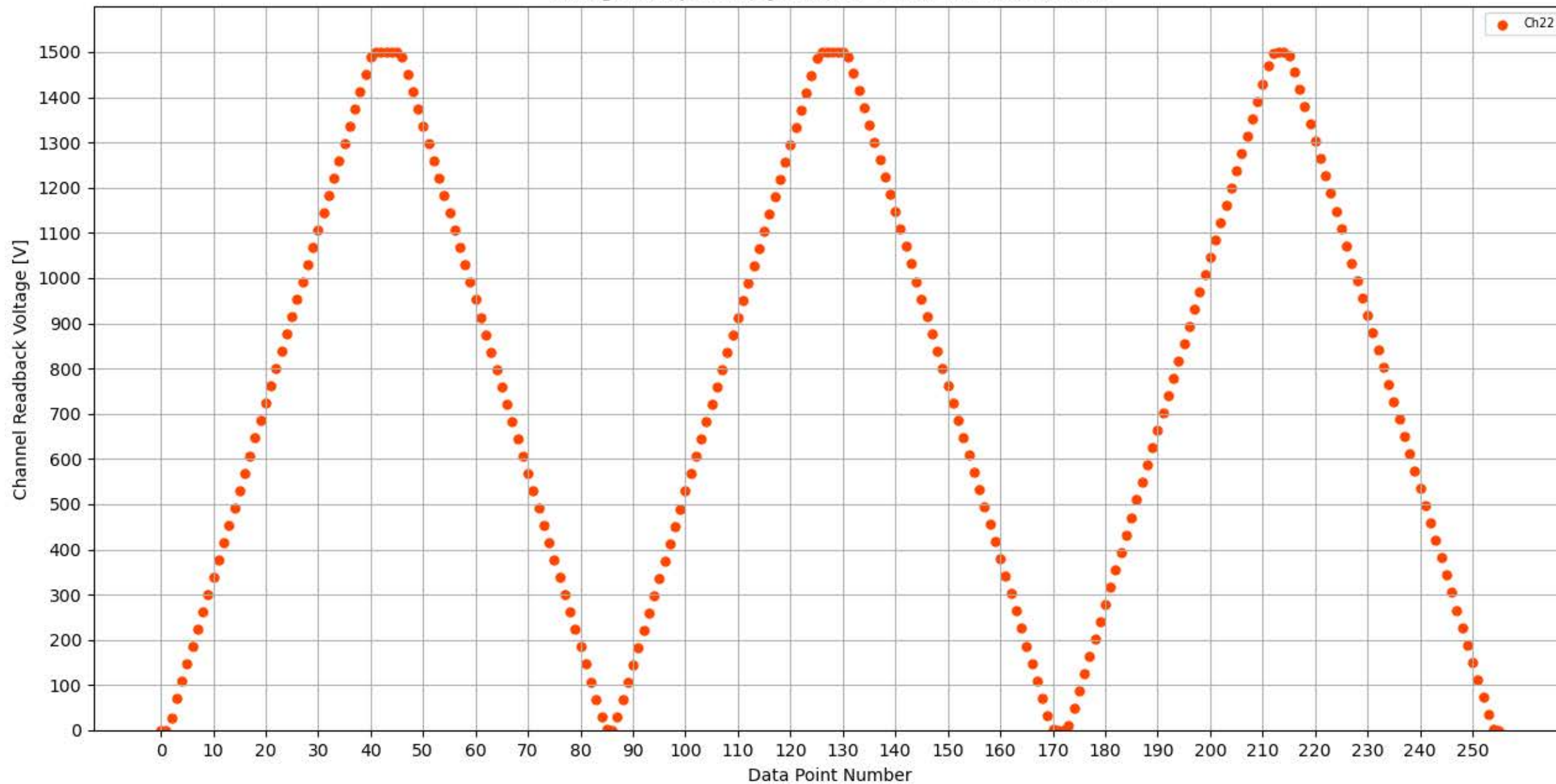
Voltage Ramp Test (Python) Bd #173, Slot #9, Ch #22
