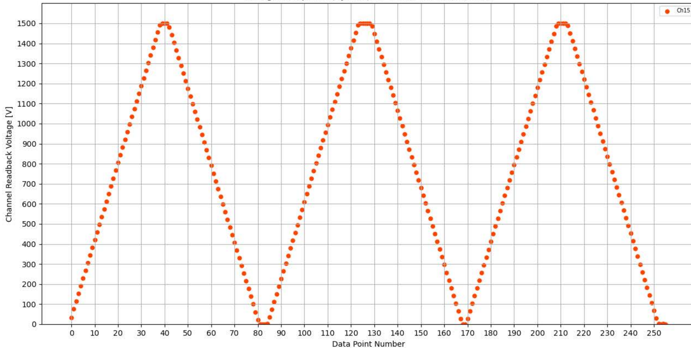
Voltage Ramp Test (Python) Bd #173, Slot #9, Ch #15
